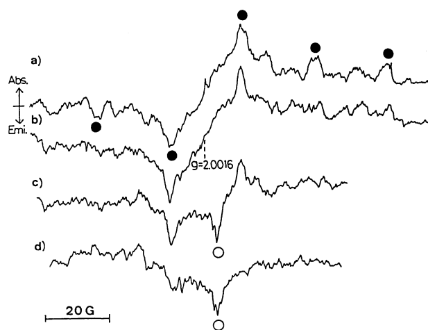
Fig. 6. CIDEP spectra of DOB in MCH at (a) room temperature, (b) -10, (c) -40, and (d) -70 °C. Marked by the solid circles in (a) are the methylcyclohexyl radical signals. In (c) and (d), the open circle indicates the benzoyl radical signal.
